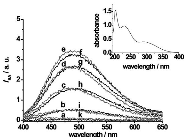
Figure 1. Intensity of the benzamide band I_{BA} of 4^{12-} in water at low (a) 4.5 \times 10^{-8} , b) 9.1 \times 10^{-7} , c) 3.9 \times 10^{-6} , d) 8.2 \times 10^{-6} , e) 1.7 \times 10^{-5} , f) 3.5 \times 10^{-5} mol L ^{-1} (gray lines) and high (g) 5.1 \times 10^{-5} , h) 8.7 \times 10^{-5} , i) 1.5 \times 10^{-4} , k) 2.7 \times 10^{-4} mol L ^{-1} (black lines) concentrations of 4 ( \lambda_{ex}=333 nm; inset: absorption spectrum of 4 ).
