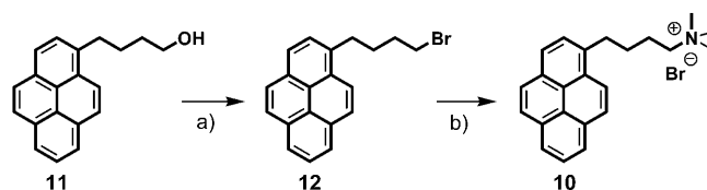
Scheme 2. Synthesis of 1-(4-trimethylammoniumbutyl)pyrene bromide ( 10 ): Reagents and conditions: a) \text{CBr}_4 , \text{PPh}_3 , \text{CH}_2\text{Cl}_2 , 6 min; b) \text{NMe}_3 , THF, 8 h.
