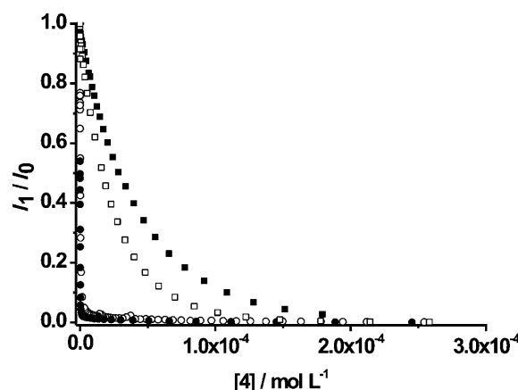
Figure 15. Intensity ratio I_1/I_0 of the pyrene-based emissions of 10 and 13 as a function of the concentration of 4 in the presence of 10 ( 6.10 \times 10^{-7} \text{ mol L}^{-1} ) at pH 7 ( \circ ) and 9 ( \bullet ) and in the presence of 13 ( 6.10 \times 10^{-7} \text{ mol L}^{-1} ) at pH 7 ( \square ) and 9 ( \blacksquare ).
