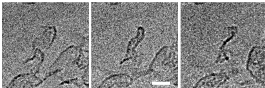
Figure 10. Cryo-TEM images showing in detail the porous membrane formed by 4 at pH 4 (cf. Figure 9) at different tilt angles ( -22.5^\circ , 0^\circ , and +22.5^\circ from left to right) revealing the membrane layer thickness of 6 nm (right) (bar: 50 nm).
