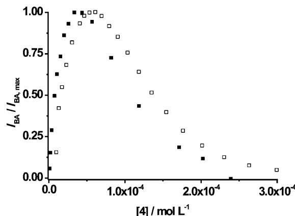
Figure 4. I_{BA}/I_{BA,max} of 4 versus the concentration of 4 at pH 7 ( \square ) and 9 ( \blacksquare ).
