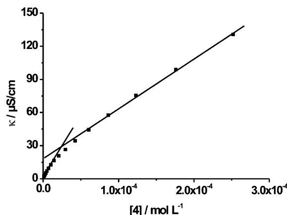
Figure 3. Variation of conductivity versus the concentration of 4^{12-} for the determination of the cmc in pure water ( \kappa=2 \mu S, T_{ref}=25 °C).
