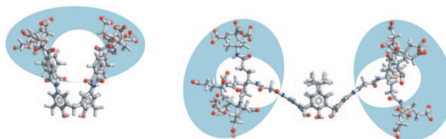
Figure 8. Spatial conformations of the head groups of 4 (left) and 1 (right) found in structurally persistent spherical micelles. The smaller space required by 4 allows denser packing of the second-generation dendritic head groups compared with the third-generation head groups in compound 1 .
