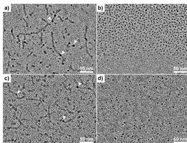
Figure 6. Typical cryo-TEM images of 4 in buffered water at different pH values and in the presence of pyrene. Pure 4 forms predominantly rodlike and spherical micellar aggregates at pH 7 (a) and only almost uniform spherical micelles at pH 9 (b). After the addition of pyrene the dimensions of the aggregates at pH 7 remain unaffected (c), whereas at basic pH the loaded micelles are less uniform providing a larger particle size distribution (d). The formation of micellar end-caps can be detected (see arrows in a and c) irrespective of the addition of pyrene.
