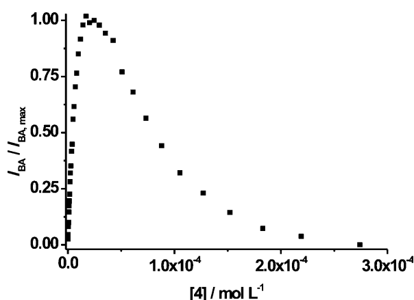
Figure 2. Intensity of the benzamide band I_{BA} of 4^{12-} at 485 nm versus the concentration of 4^{12-} in pure water ( \kappa=2 \mu S, \lambda_{ex}=333 nm).
