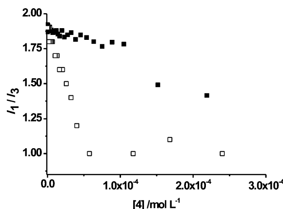
Figure 13. I_1/I_3 of pyrene versus the concentration of 4 at pH 7 ( \square ) and 9 ( \blacksquare ) in the presence of pyrene ( 6.10 \times 10^{-7} \text{ mol L}^{-1} ).
