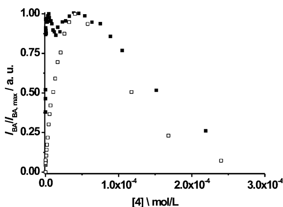
Figure 12. Intensity of the benzamide band I_{\text{BA}} of 4 versus the concentration of 4 in the presence of pyrene ( 6.10 \times 10^{-7} \text{ mol L}^{-1} ) at pH 7 ( \square ) and 9 ( \blacksquare ).
