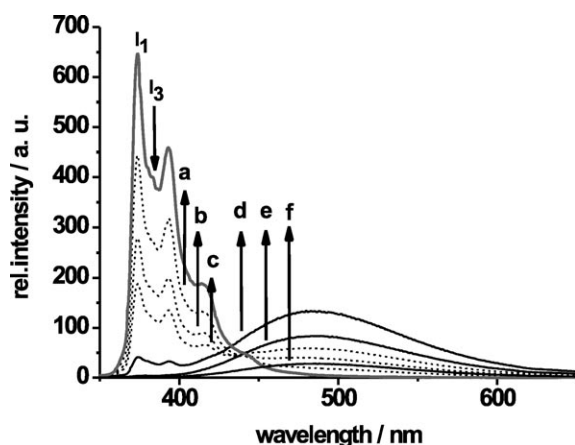
Figure 11. Fluorescence spectra of 4 in the presence of pyrene ( 6.10 \times 10^{-7} \text{ mol L}^{-1} ) at varying concentrations of 4 (a) 1.9 \times 10^{-6} , b) 4.8 \times 10^{-6} , c) 7.2 \times 10^{-6} (dashed lines), d) 8.2 \times 10^{-6} , e) 3.1 \times 10^{-5} , f) 5.3 \times 10^{-5} \text{ mol L}^{-1} (black lines)) and of 6.0 \times 10^{-7} \text{ mol L}^{-1} pyrene (gray line) in buffered solution at pH 7 ( \lambda_{\text{ex}} = 333 \text{ nm} ).
