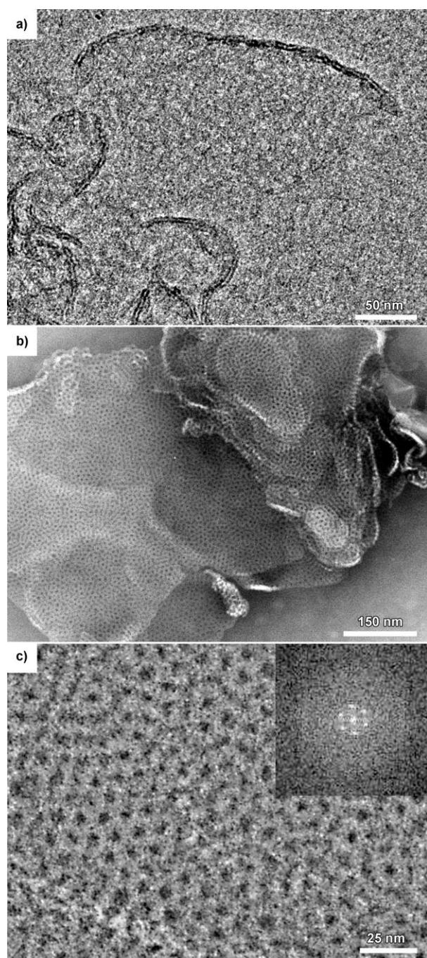
Figure 9. a) Cryo-TEM image and b) negatively stained (phosphotungstic acid) preparation of 4 at pH 4. A porous membrane is formed that shows pores of 5.0 nm diameter in a hexagonal arrangement, as shown by the magnified image and its corresponding Fourier transform in (c).
