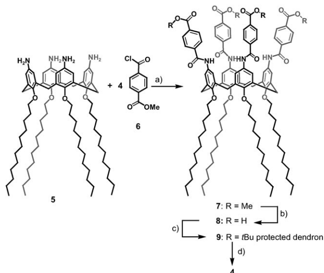
Scheme 1. Synthesis of the terephthal calixarene 4 . Reagents and conditions: a) i. \text{SOCl}_2 , DMF, 70^\circ\text{C} , 4 h; ii. THF, -10^\circ\text{C} to room temperature; b) LiOH, \text{H}_2\text{O} , THF, 6 h, 60^\circ\text{C} ; c) EDC, HOBT, DMAP, DMF, 0^\circ\text{C} to room temperature, 72 h; d) formic acid.
